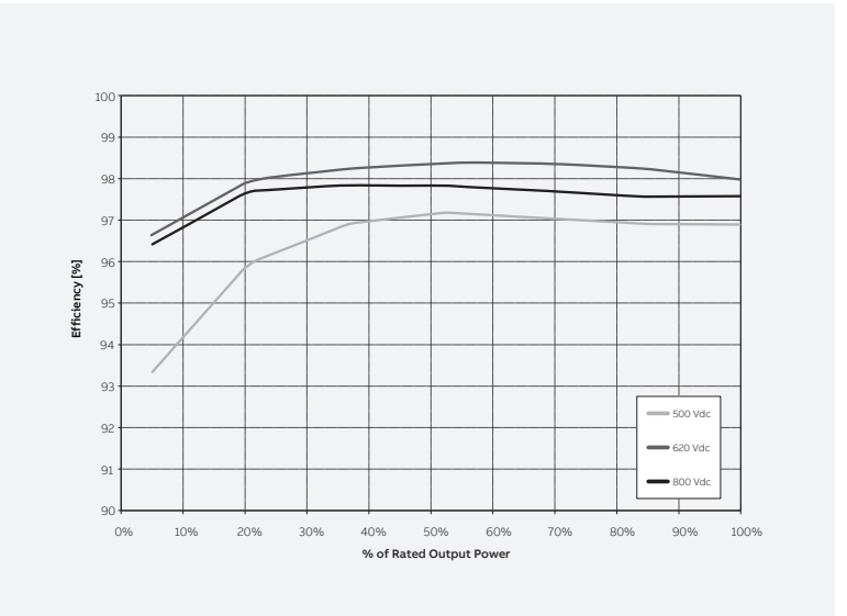
Efficiency curves of TRIO-27.6-TL-OUTD
