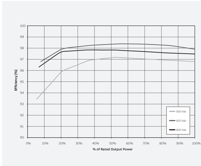
Efficiency curves of TRIO-20.0-TL-OUTD
